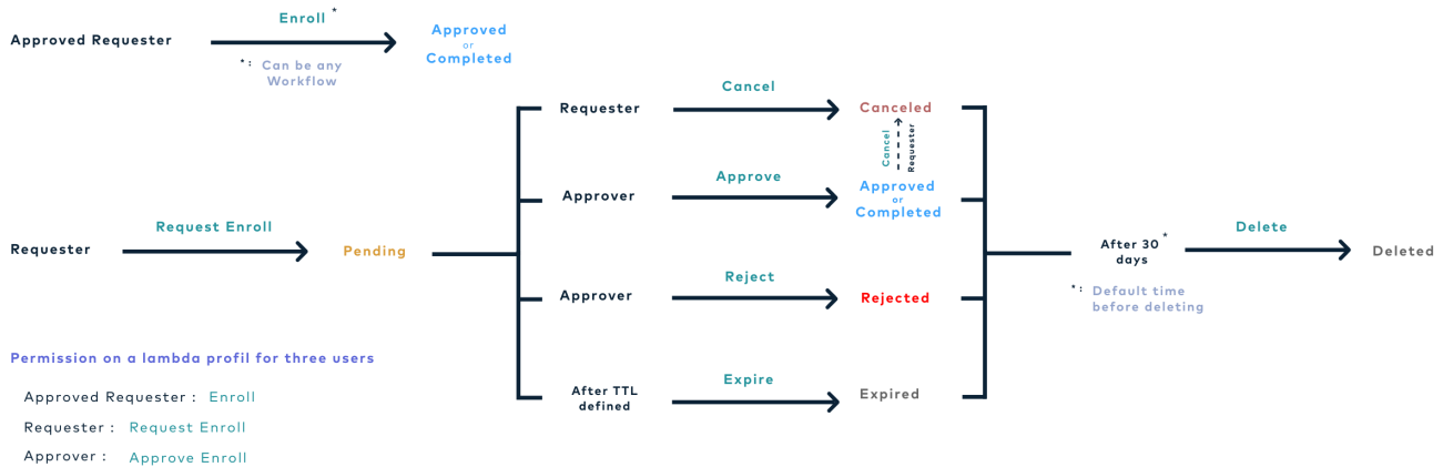
Figure 1. Request Workflow
